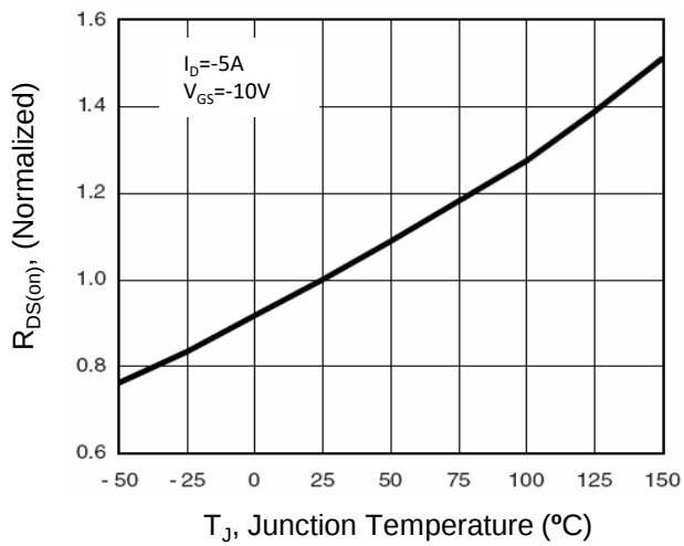
Figure 7. Drain-Source On-Resistance
